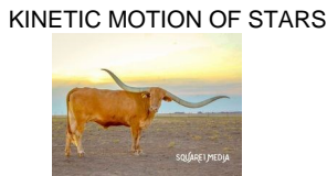
KINETIC MOTION OF STARS
